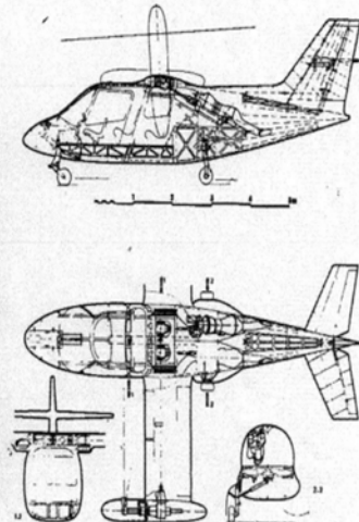
Figure 201 - Convertible X 910
