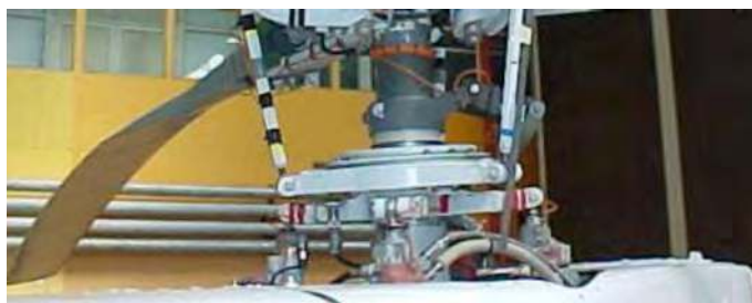
Figure 158 - EC130-B4 Plateau cyclique
