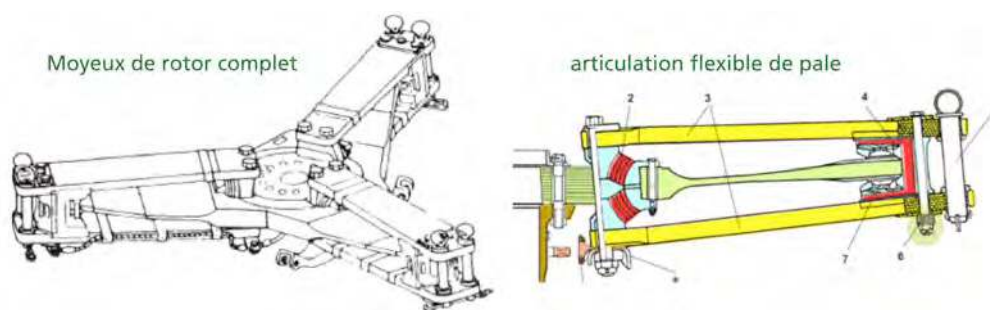
Figure 139 - Moyeu Starflex
